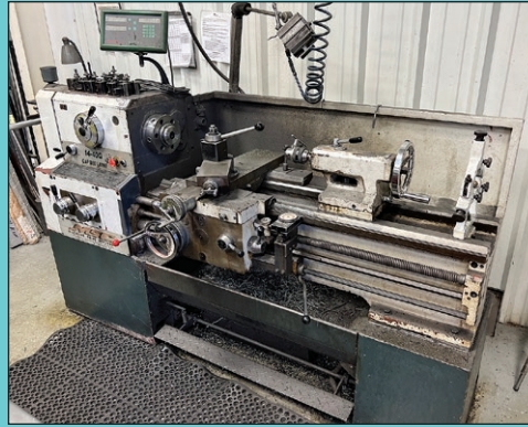
14" x 40" MSC 14-40G Gap Bed Lathe w/ DRO
